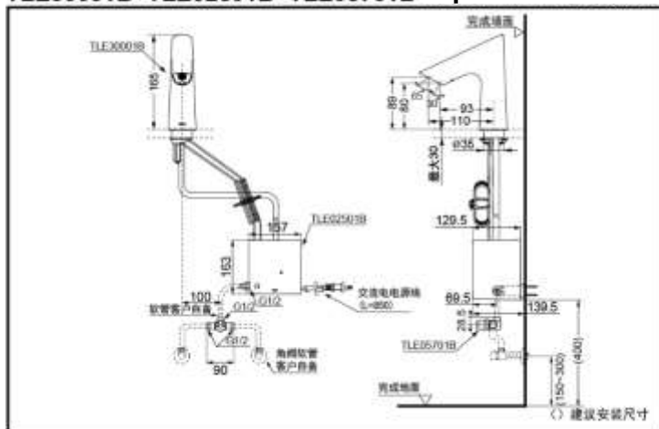
TLE30001B+TLE02501B+TLE05701B Aqua-auto faucet EWATER(thermal)
