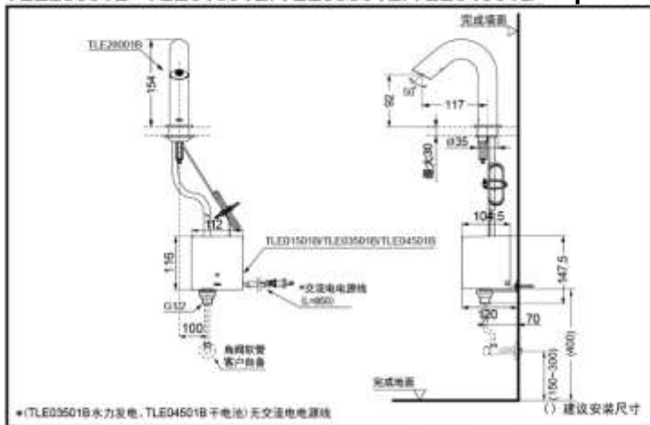
TLE28001B+TLE01501B/TLE03501B/TLE04501B +TLE05701B Aqua-auto faucet(thermal)
