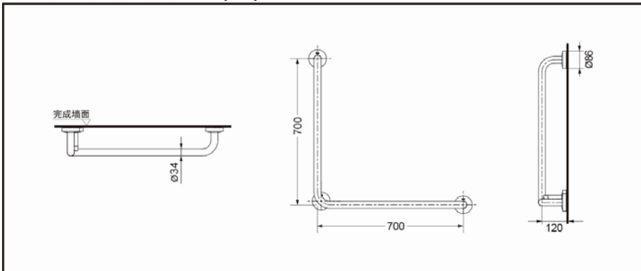
T112CL10 V2NW Multipurpose handrail
